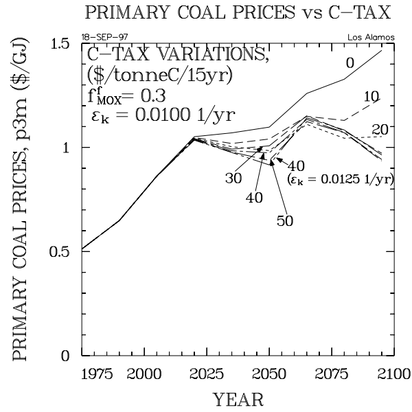
Figure 47C. Primary fossil-energy world-market prices required for market-clearing for a range of carbon-tax scenarios, as well as for the conditions describing the basecase GCC scenario: primary coal world-market-clearing prices.
