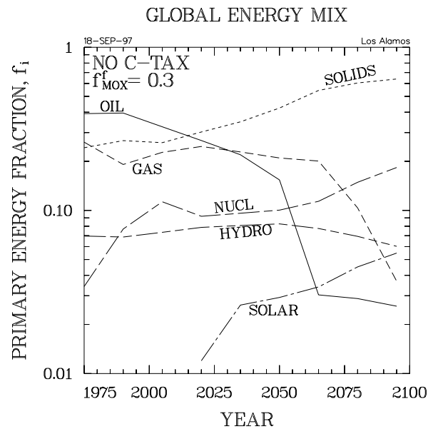
Figure 4B. Cumulative evolution of global primary energy mix for the Basis Scenario (solids = coal + biomass): Primary energy fractions.
