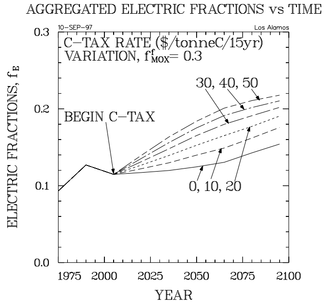
Figure 21. Fraction of total primary energy supplied by electricity as a function of time and carbon tax rate, starting in 2005.
