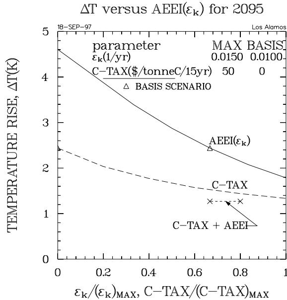
Figure 41. Global temperature rise as a function of relative changes in demand-side ( \epsilon_k ) and supply-side (carbon tax rate) scenario attributes, with reference and basis-scenario values of each indicated; also shown is the combined AEEI + C-TAX case.
