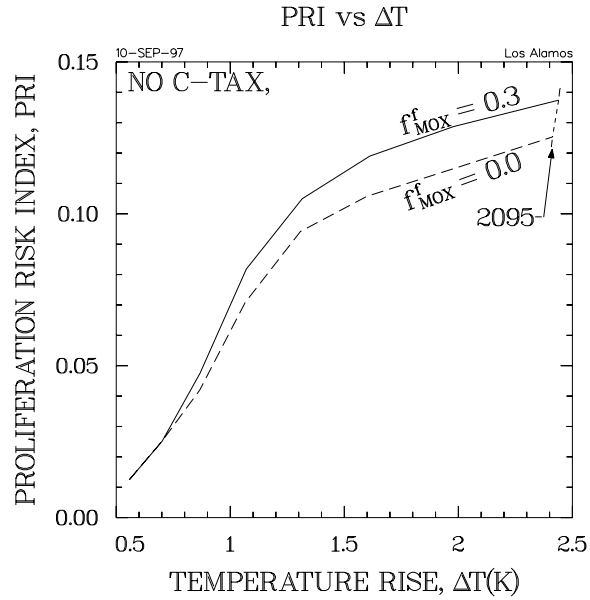
Figure 12. Correlation of proliferation-risk index with average global temperature rise for case without carbon tax imposed; comparison of PRI impacts of plutonium recycle (e.g., f_{\text{MOX}}^f = 0.0 versus 0.30) is shown.
