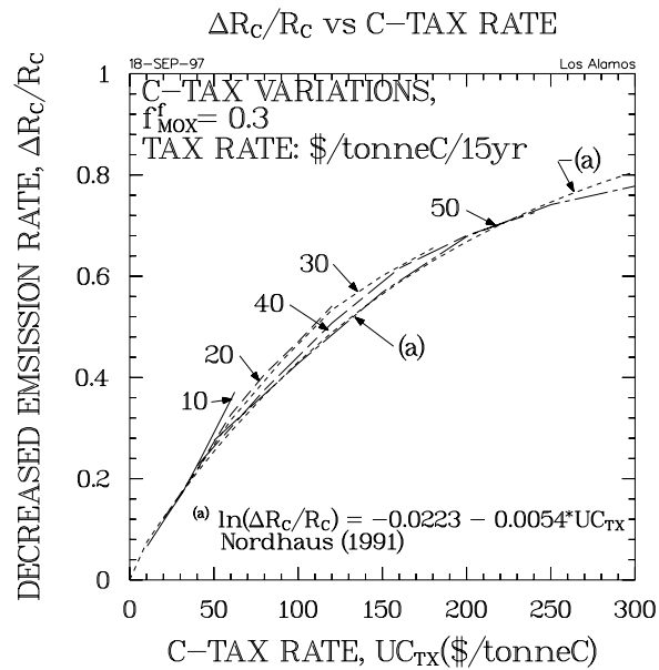
Figure 25. Decrease in atmospheric carbon emission rate as a function of carbon tax for a range of carbon tax rates; a regression fit to a number of model predictions 38 is also shown.
