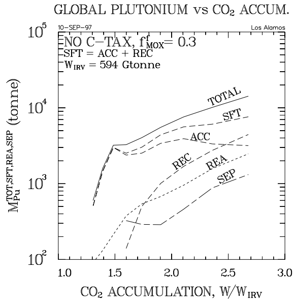
Figure 11A. Correlation of proliferation-risk index for no carbon taxes with atmospheric CO 2 (carbon) accumulation relative to pre-industrial levels ( W_{IRV} = 594 Gtonne).
