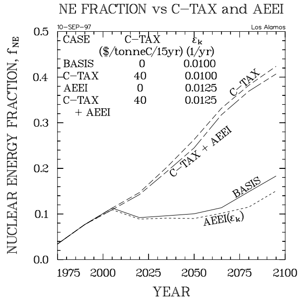
Figure 34. Nuclear energy fraction of primary energy (same basis) as a function of time for a combination carbon tax rate and AEEI, showing relative impacts of supply-side (carbon tax) and demand-side (AEEI) scenario attributes.
