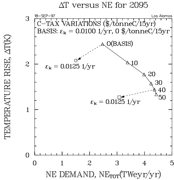
Figure 43A. Dependence of global temperature rise on carbon-tax-induced (supply-side) nuclear-energy demand, showing impact of demand-side increases in AEEI for the Basis Scenario (no carbon taxes) and for a case where the carbon tax is imposed at a rate of 40 $/tonneC/15yr.
