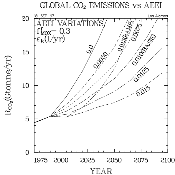
Figure 17. Carbon-dioxide (carbon) emission rate as a function of time and AEEI; the \epsilon_k = 0.015(\text{RAMP}) case starts ramping from the indicated value in 2005 and linearly decreases to zero by 2095.
