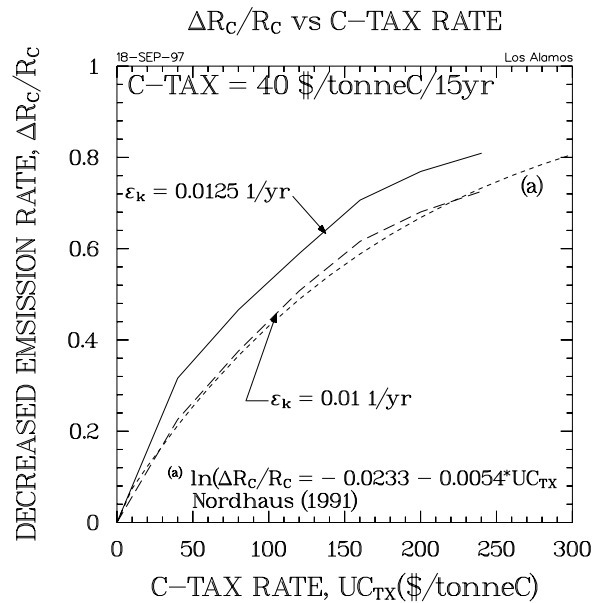
Figure 37. Impact of AEEI on effectiveness of carbon taxes in reducing emissions of atmospheric carbon for a carbon tax rate of 40 $/tonneC/15yr; shown also is a regression fit to a number of model predictions. 38
