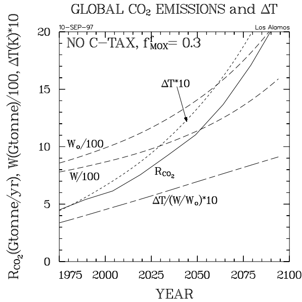
Figure 9. Time dependence of total CO 2 (carbon) emission, integrated emissions, atmospheric accumulation of emissions, and corresponding global average temperature rise, as determined from the linear integral-response model; 15,16 results applied to the zero carbon-tax basis case. 24
