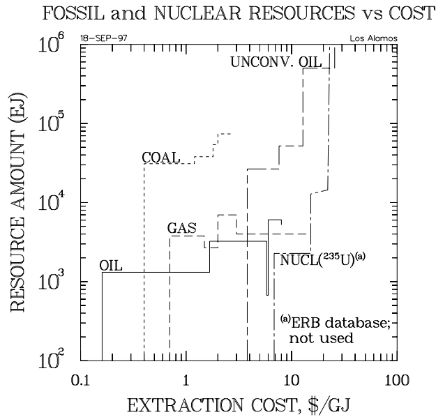
Figure 45B. Fossil energy resources used in the ERB model; 5 the uranium resource reported here has been replaced with that of Ref. 33: resource as a function of extraction cost, per the Ref.-5 definitions.
