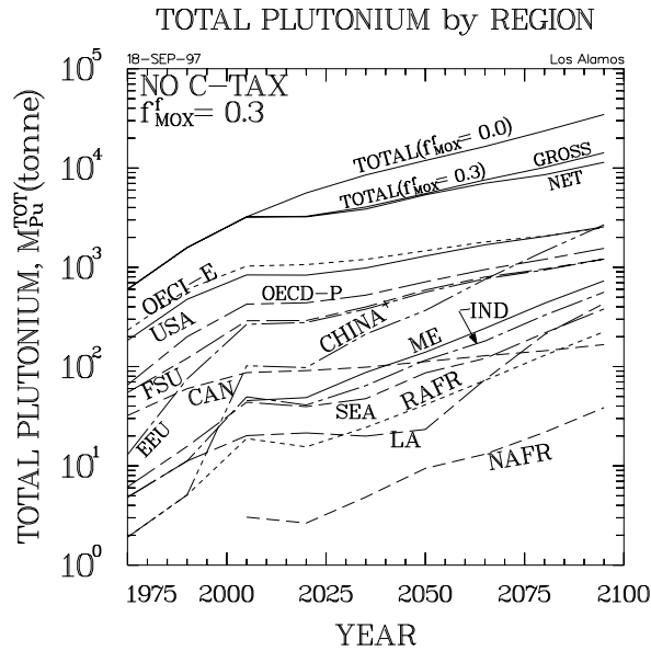
Figure 7. Region breakout of total accumulated plutonium for the Basis Scenario.
