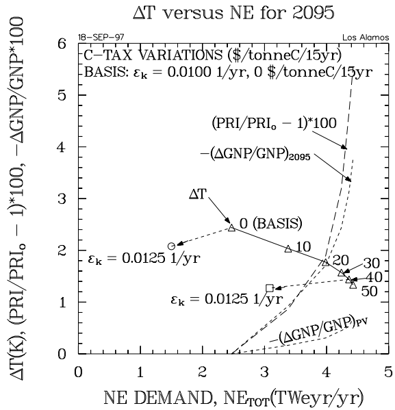
Figure 43B. Dependence of global temperature rise on carbon-tax-induced (supply-side) nuclear-energy demand, showing impact of demand-side increases in AEEI for the Basis Scenario (no carbon taxes) and for a case where the carbon tax is imposed at a rate of 40 $/tonneC/15yr; also shown is the increase in PRI relative to the Basis Scenario as well as the relative decrease in GNP.
